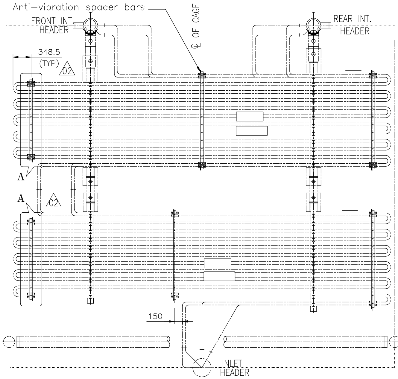
HORIZONTAL COILS (ANTI-VIBRATION BAR DETAIL)
